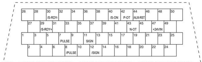
\Sigma -V Series (50 Pins)
