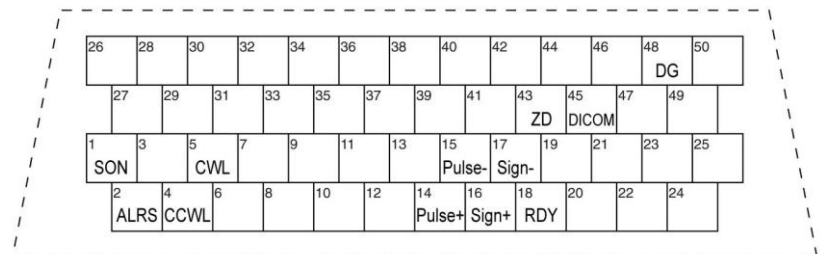
SR, TSDA, SD (50 Pins)
