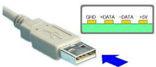
USB-A Connector Side
