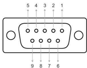
RadonixPC+ (DB9FM) Side
