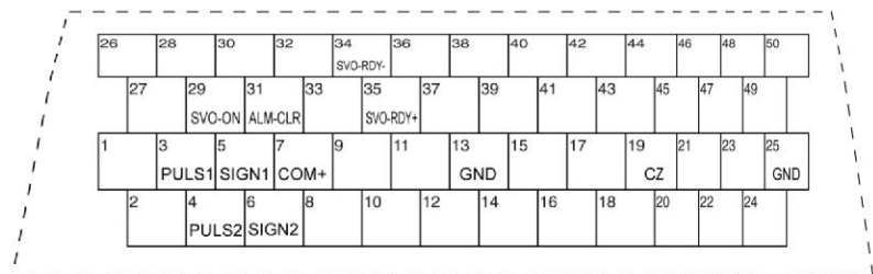
KSDG (50 Pins)
